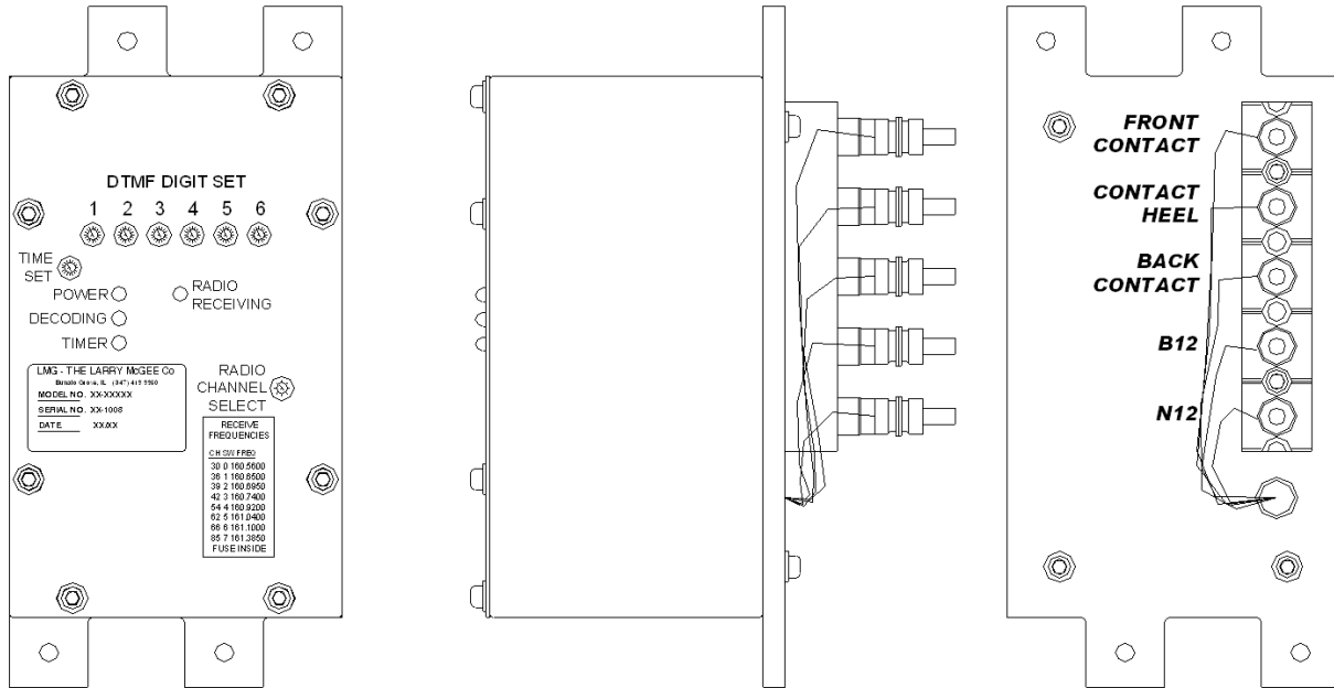
Radio DTMF Activator—Rack-Mounting Version 14-99005Ayz
