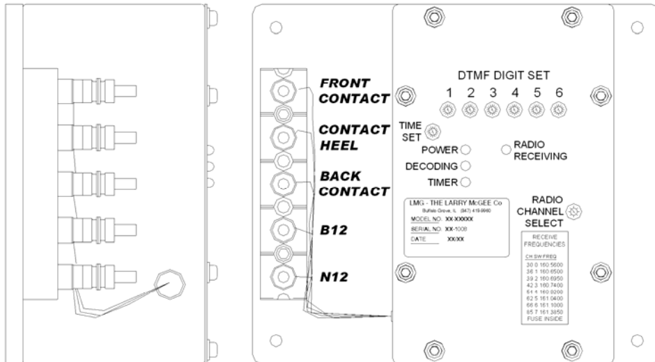
Radio DTMF Activator—Wall Mounting Version 14-99005V2-Byz
